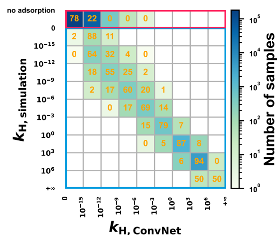
Fig. 6 Normalized confusion matrix showing the percentage of zeolites from a given target group ( k_H for n-octadecane adsorption from Monte Carlo simulations; y axis) in different predicted groups of k_H using the best ResNet18 model. The background color of each grid indicates the number of zeolites represented. For comparison, the ResNet18 model was also applied to the zeolites with k_H = 0 that were not included in the training set. The predictions for these unseen zeolites are shown in the top row.
