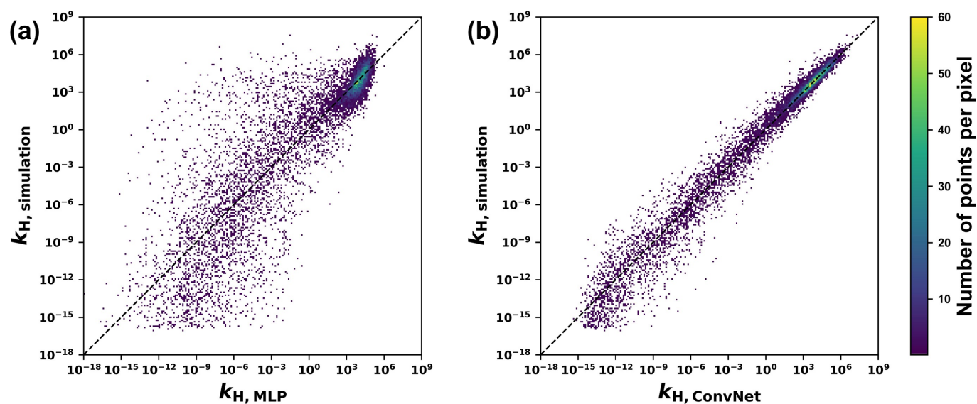
Fig. 5 Scatter plot of the testing performance, comparing Henry's constants for n-octadecane adsorption (unit: mol/kg/MPa) predicted by MLP (a) and ResNet18 (b) and target values from Monte Carlo simulations. Color indicates the number of points per pixel.
