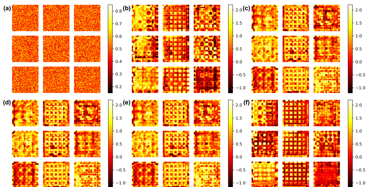
Fig. 9 Feature visualization showing (a) a random input and (b-f) input grids that strongly activate a particular feature map in the last Conv layer of the best ResNet18 model. In each subplot, the top, center, and bottom rows show 2D slices at x , y , and z = 1 (left), 25 (middle), and 50 (right).
